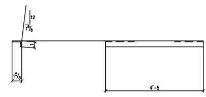
3 - TREADS - 54F
