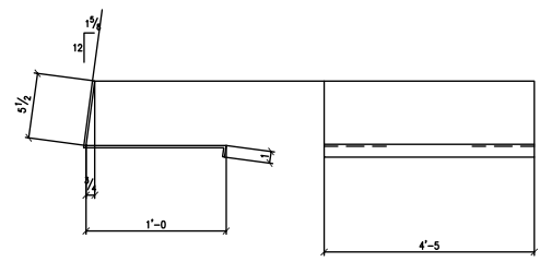
30 - TREADS - 54D
